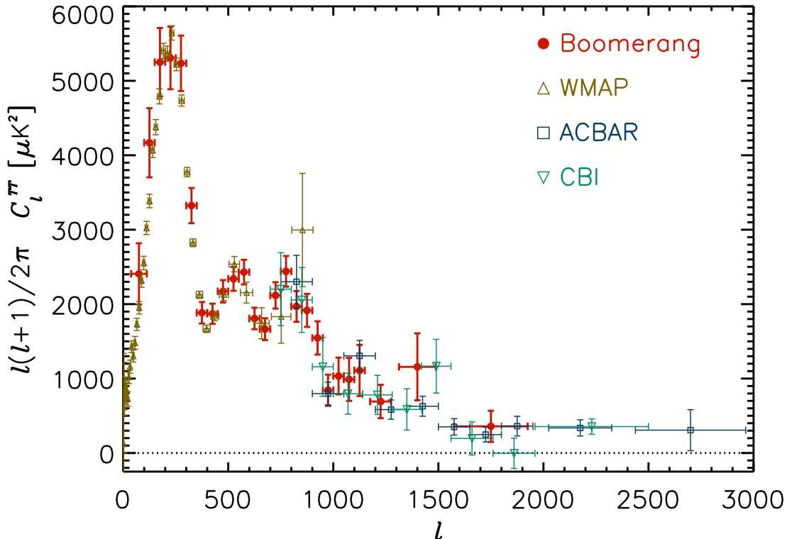
FIG. 5.— A comparison of recently published CMB power spectra, C_l^{\text{TT}} , [the data shown are from Hinshaw et al. (2003); Kuo et al. (2004); Readhead et al. (2004), in addition to B03]. The data shown are derived from independent measurements that span two orders of magnitude in electromagnetic frequency (20-200 GHz), employ both single dish and interferometric instruments, and operate from terrestrial, balloon-borne, and orbital platforms. The remarkable degree of accord between such a diverse set of measurements is indicative of the maturity of the observational field.
