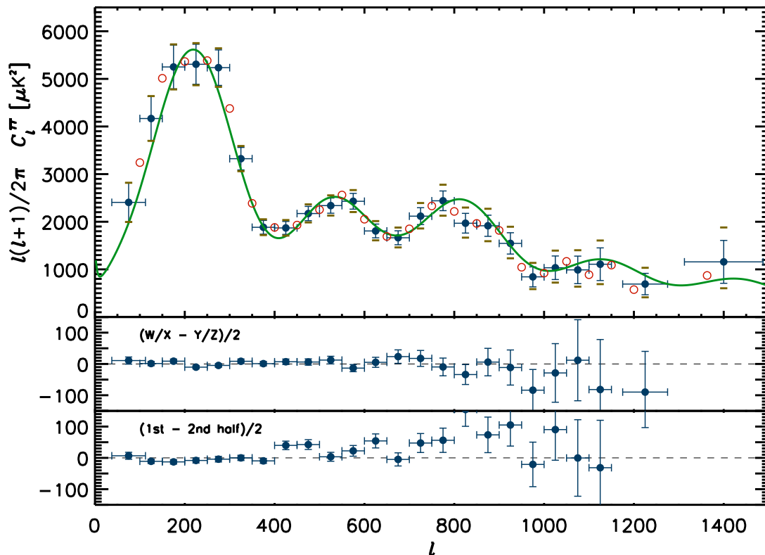
FIG. 3.— The temperature angular power spectrum, C_l^{TT} , derived from the B03 data. The red points represent an alternate binning, and should not be interpreted as having statistical weight beyond that of the nominally binned data, which are shown with errorbars. The anti-correlations between neighboring bands range from the twelve to twenty percent level. The envelope of the beam uncertainty is indicated by ticks bracketing the one sigma errorbars for each of the bandpower estimates. As discussed in Section 3.5, these limits indicate the amount of “tilt” to the spectrum that is allowed by the beam uncertainty, and should not be interpreted as an additional uncorrelated error in each bin. The solid green line is the concordance \Lambda CDM model which best fits all published CMB data, including the B03 temperature and polarization results. The power spectra of the consistency checks described in the text are shown in the lower two panels.
