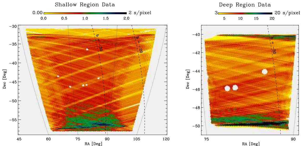
FIG. 1.— The left and right panels show the sky coverage obtained during the January 2003 flight of BOOMERANG. The integration times per 3.4' pixel are shown for the shallow and deep data subsets described in the text. Galactic latitude contours of b = \{-30, -20\} are shown for reference. Approximately 75 hours of observation are devoted to the shallow region, with an additional 120 hours concentrated in the central deep field. The cross-linking of the scans due to sky rotation is evident in the diagonal striping of the coverage, which has a \approx 20^\circ opening angle. Known extragalactic point sources, shown masked in these plots, are excluded from the analysis.
