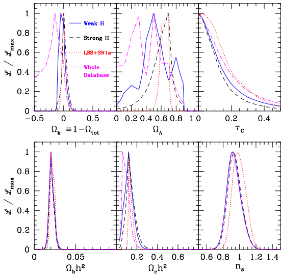
Fig. 4.— Likelihood functions for a subset of the priors used in Table 4. \Omega_b h^2 , and n_s are well constrained, even under the “whole database” case, and are insensitive to additional priors. \Omega_{\text{tot}} is poorly constrained over the whole database, but when the weak priors are applied, it becomes stably consistent with the flat case. With the weak priors, \Omega_\Lambda and \Omega_c h^2 are poorly constrained, but become significant detections with the addition of the other priors considered. For all cases, \tau_c is poorly constrained, but does prefer low values.
